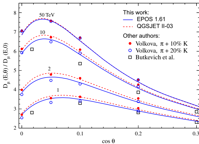
Fig. 17. Zenith-angle enhancement of the muon flux, D_\mu(E, \theta)/D_\mu(E, 0) , calculated with the EPOS (solid lines) and QGSJET II (dashed), both for the ATIC-2 primary spectrum. Symbols present the calculations of [22] (squares) and [95] (circles). Numbers above curves are the muon energies in TeV.
