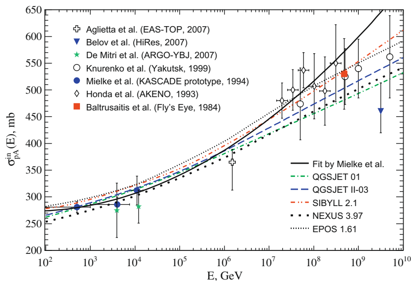
Fig. 3. Proton–air inelastic cross-section: the model predictions vs. experiments [51–57]. Solid line presents the fit \sigma_{pA}^{in} = 290 - 8.7 \log E + 1.14 \log^2 E [51].
