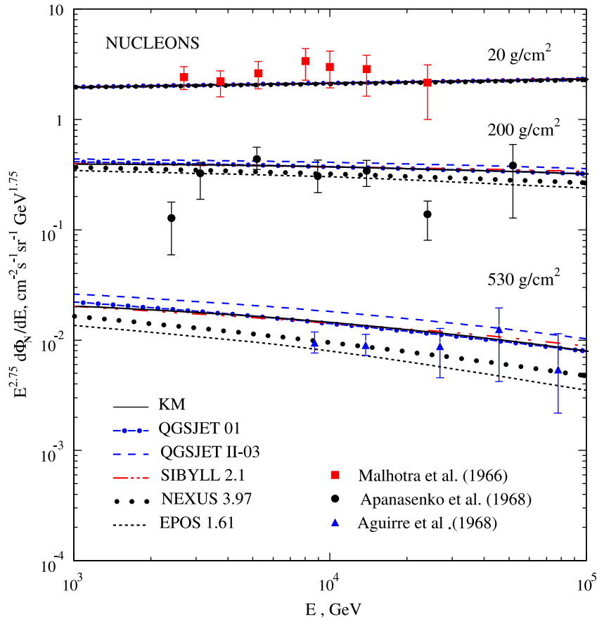
Fig. 4. Nucleon energy spectra at three atmospheric depths, computed with the GH primary spectrum and various hadronic models. The experimental data are from Refs. [63–65].
