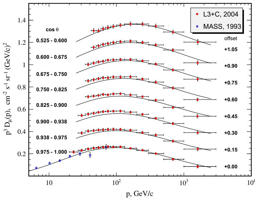
Fig. 16. Comparison of the predictions for near-vertical muon fluxes with the data of the L3 + Cosmic experiment. The computations are made for the ATIC-2 primary spectrum with usage of KM. The MASS data are added to view the low-energy junction.
