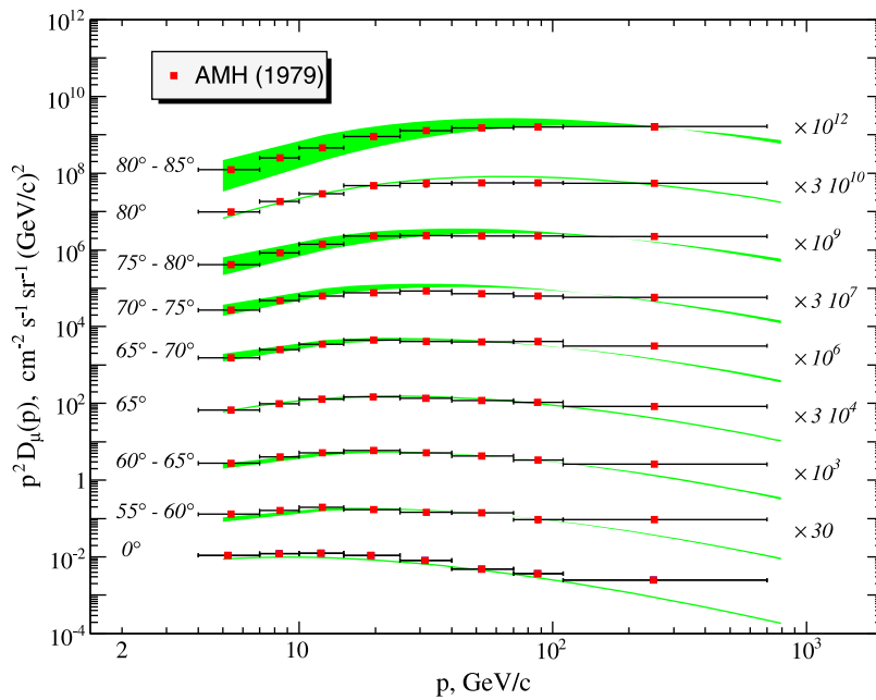
Fig. 12. The muon flux calculated for wide range of zenith angles in comparison with the data of AMH [87] magnetic spectrometer. Calculations are performed for the ATIC-2 primary cosmic-ray spectra and KM model. The bands show the calculated flux spread due to uncertainties in zenith angles.
