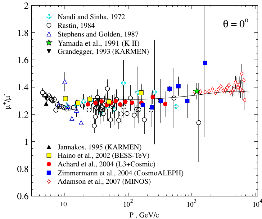
Fig. 18. Muon charge ratio at sea level calculated with KM model for the ATIC-2 primary spectra. The data of experiments are taken from Refs. [13,14,96–102].
