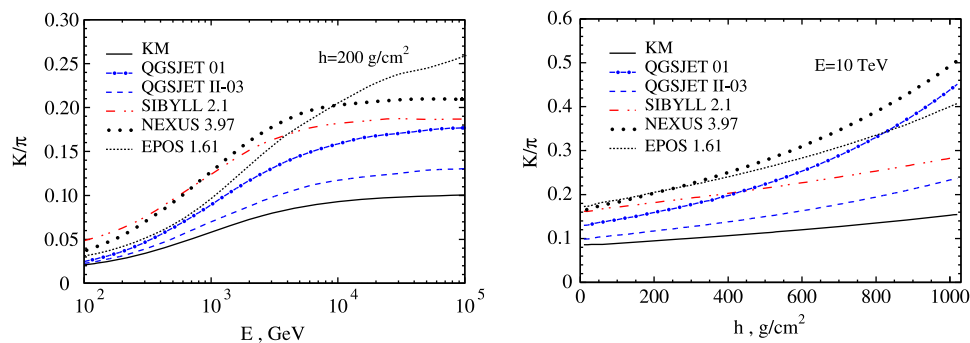
Fig. 9. Charged K/\pi -ratio, depending on the energy, calculated for the atmospheric depth of 200 \text{ g cm}^{-2} (left plot), and that at 10 \text{ TeV} unfolded along the atmospheric depth (right plot). GH primary spectrum is used.
