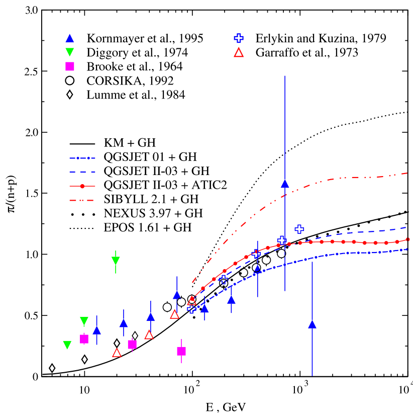
Fig. 8. The ratio \pi/(p+n) calculated at sea level with the set of hadronic models. The ATIC-2 primary spectrum and GH parameterization are used. Experimental data (closed symbols) and calculations of other works (open symbols) are taken from Ref. [66].
